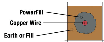
HORIZONTAL CONSTRUCTION
